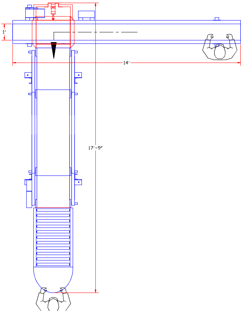
MODEL BC14-LP CONVEYOR
